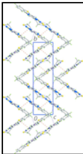
Fig. 3. A view in projection down the a axis of the unit-cell contents of (I). The C—H...N, C—H... \pi and \pi ... \pi interactions are shown as blue, purple and orange dashed lines, respectively.
