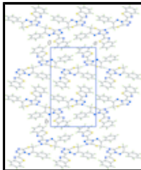
Fig. 2. Supramolecular chains in (I) mediated by C—H...N interactions (blue dashed lines).
